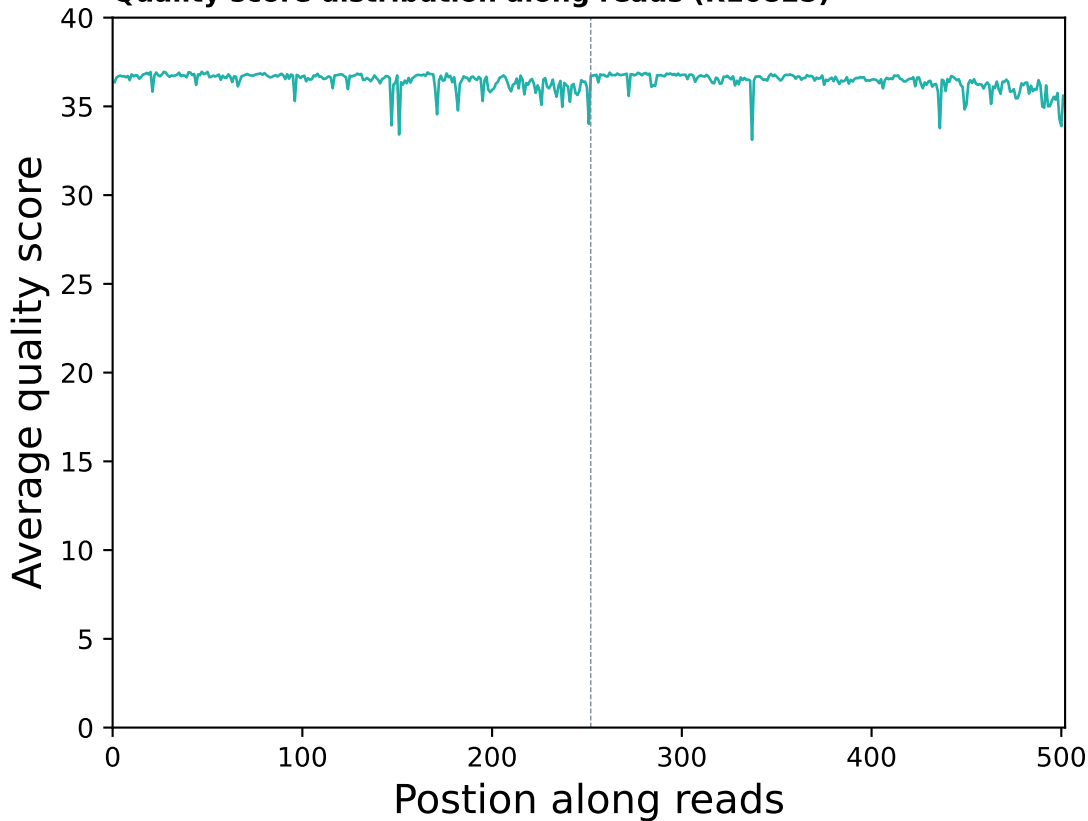
Quality score distribution along reads (R10825)
